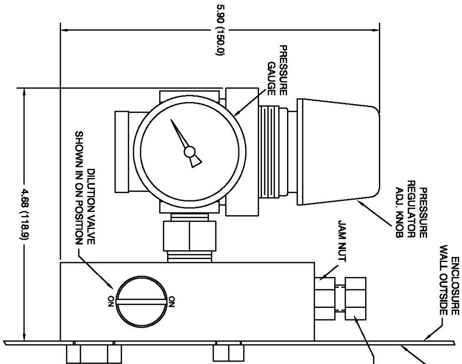
FRONT VIEW
